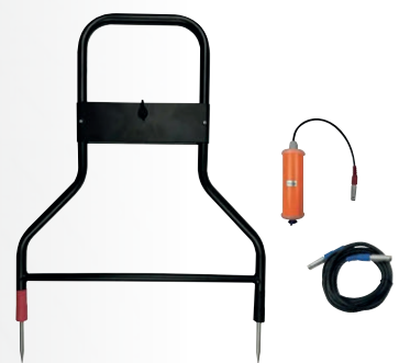
Cable Fault Locator A-Frame G9325
