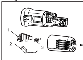
1. Brush Holder 2. Carbon Brush 3. Coil Spring
