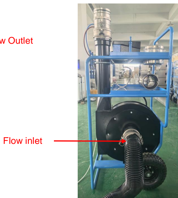
Low-flow Duct testing under Negative pressure
