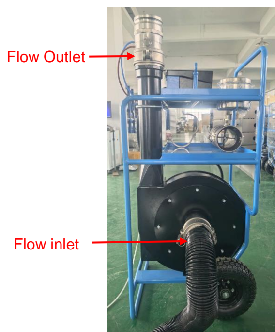
High flow Duct testing under Negative pressure
