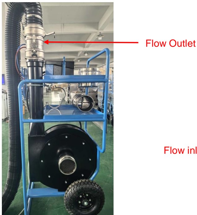
Low-flow Duct testing under positive pressure
