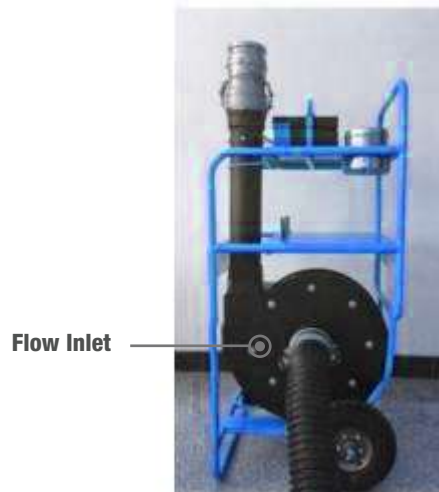
Low-flow duct testing under negative pressure
