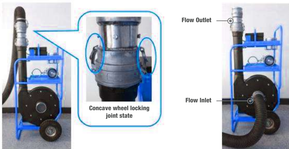
High-flow duct testing under positive pressure
